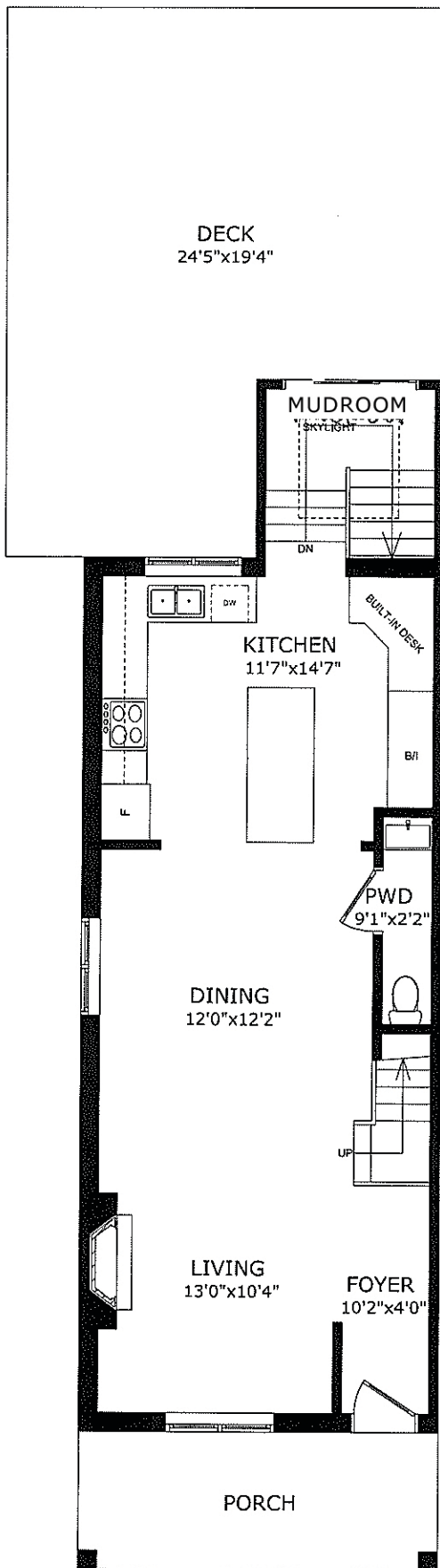
MAIN FLOOR
