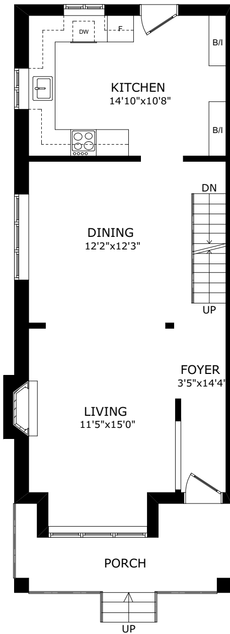
MAIN FLOOR
