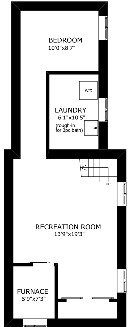
BASEMENT
