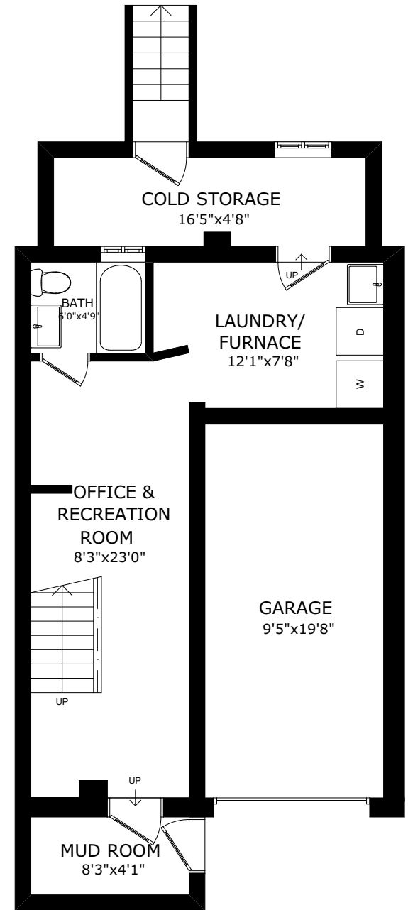
BASEMENT
