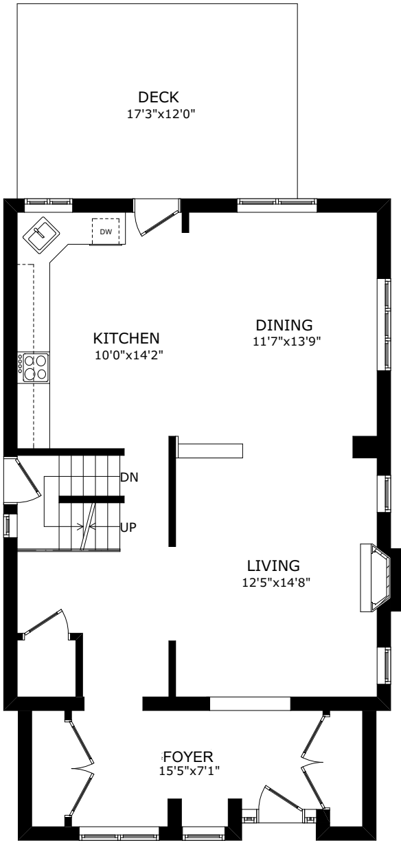
MAIN FLOOR
