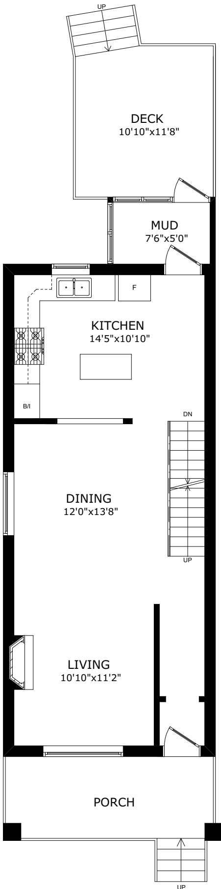
MAIN FLOOR
